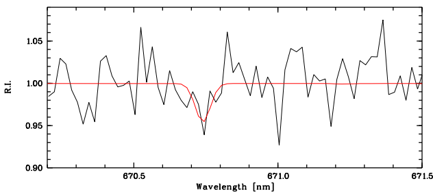
Fig. 2 (online colour at: www.an-journal.org ) The fit of the Li doublet at 670.7 nm with a grid of ATLAS + SYNTH profiles. As evident from the feature on the blue side of the Li, the Li line is comparable with the noise of the spectrum.
