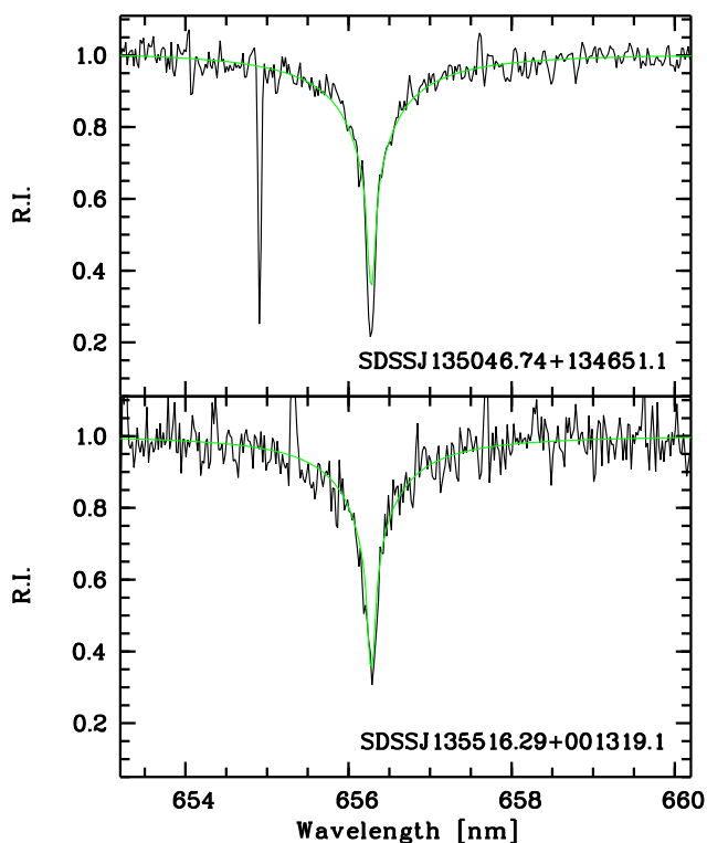
Fig. A1 (online colour at: www.an-journal.org ) The X-shooter spectrum of SDSS J135046.74+134651.1 (solid black) with the best fitting CO 5 BOLD profile ( T_{\text{eff}} = 6420 K, solid green) in the top panel and the same for SDSS J135516.29+001319.1 ( T_{\text{eff}} = 6288 K, solid green) in the bottom panel .
