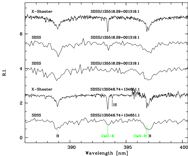
Fig. 1 (online colour at: www.an-journal.org ) The SDSS spectra of the program stars in the region around the Ca II K line compared to the X-shooter spectra. The fact that this line is weaker than the neighbouring hydrogen lines is a diagnostic for extremely low metallicity. In the X-shooter spectrum of SDSS J135046.74+134651.1 we labelled “IS” the weak interstellar Ca II K line.
