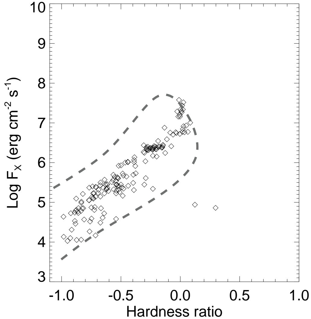
Fig. 3.— Results from Marino et al. (2001) about dF7-dK2 stars, shown similarly to Fig. 1.
