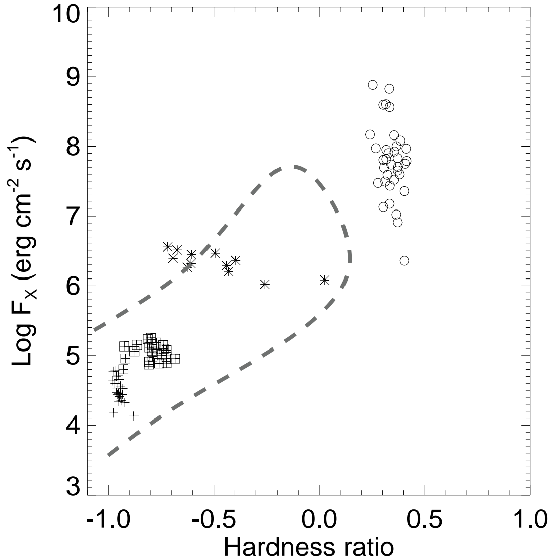
Fig. 5.— F_X - HR diagram of various kinds of structures present in the solar corona: crosses - background corona; squares - active regions; asterisks - cores of active regions; circles - flares. Data on flares are from Reale et al. (2001), all the others are from Orlando et al. (2001).
