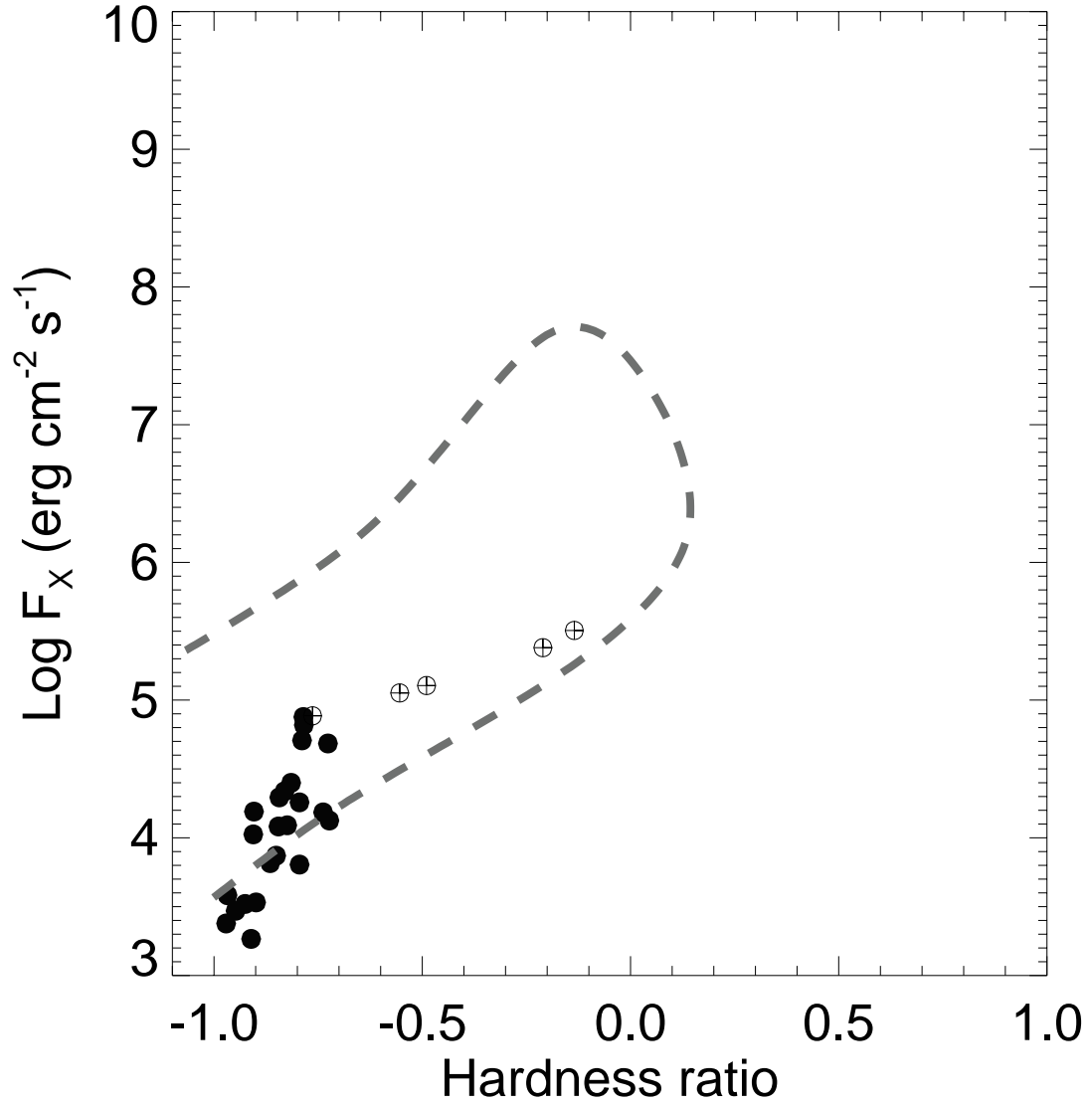
Fig. 4.— F_X -HR diagram of the whole solar corona along the solar cycle. The data points yield F_X and HR values averaged over the whole Sun; filled circled: the solar cycle from maximum (highest values) to minimum (lowest ones); circles with a cross: the whole solar corona during an X-9 flare (i.e. the evolution of the flare plus the steady non-flaring corona). Data are from Peres et al. (2000), from Orlando et al. (2001), and from Orlando et al. (2004).
