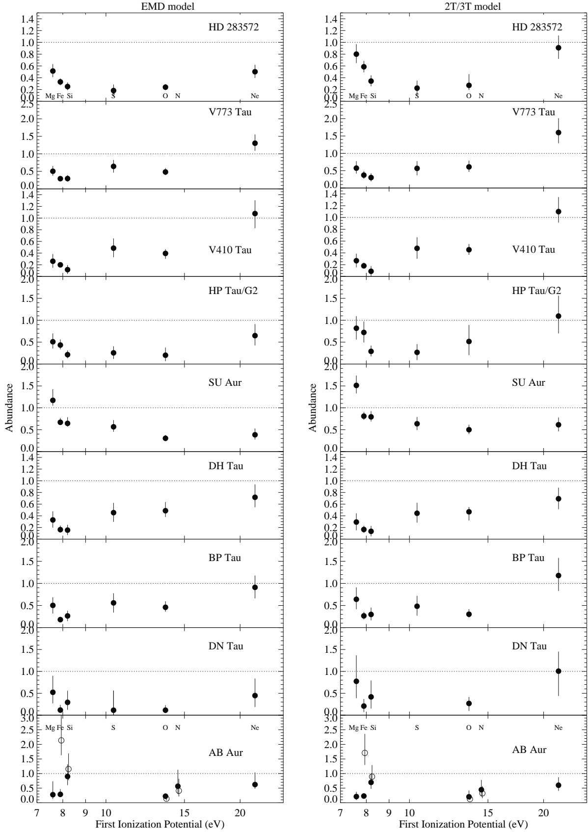
Fig. 5. Element abundances normalized to solar photospheric values (Anders & Grevesse 1989 and Grevesse & Sauval 1999 for Fe) derived from the EMD and 3T fits. Open circles for AB Aur: values normalized to the AB Aur photospheric abundances (Acke & Waelkens 2004).
