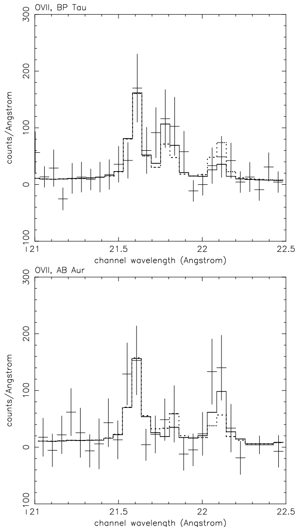
Fig. 6. Fit of the O VII triplets using variable electron density. Top panel, BP Tau: The best fit for n_e = 3.4 \times 10^{11} cm ^{-3} is plotted as a solid histogram, while the lower density limit ( n_e = 6.4 \times 10^{10} cm ^{-3} , 90% confidence) is shown by the dotted line. Bottom panel, AB Aur: The solid histogram gives the best fit ( n_e \lesssim 10^{10} cm ^{-3} ), while the dotted histogram is for the 90% upper limit to n_e ( n_e < 1.3 \times 10^{11} cm ^{-3} ).
