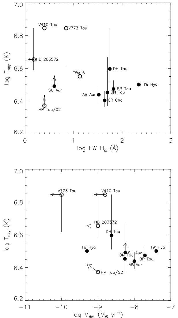
Fig. 9. Temperature corresponding to the observed \text{O VII}/\text{O VIII} count ratio as a function of H\alpha equivalent width (top) and as a function of the accretion rate \dot{M} (bottom). Errors in \log T_{\text{oxy}} are 1\sigma .
