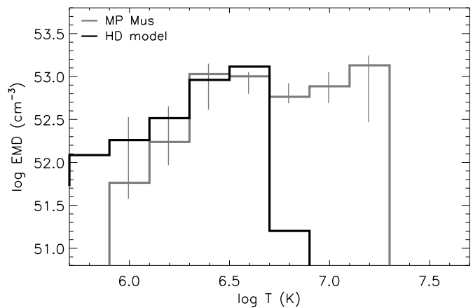
Fig. 7. EMD of MP Mus derived from the RGS line fluxes, and the EMD derived from hydrodynamical simulations of the accretion shock by Sacco et al. (2008a).
