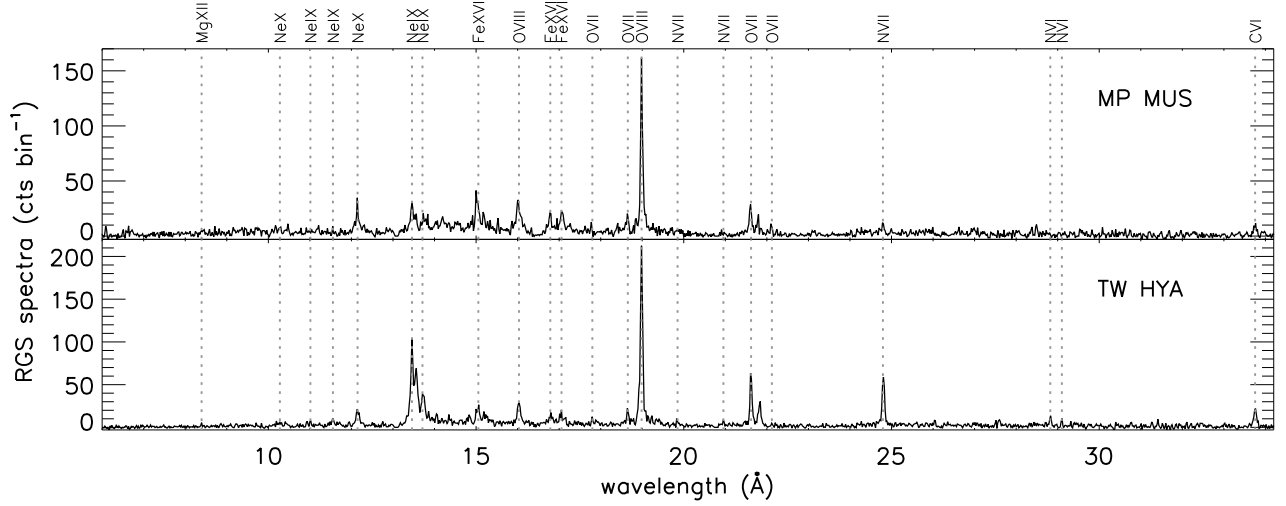
Fig. 1. RGS spectra of MP Mus and TW Hya. Each spectrum was obtained by adding RGS1 and RGS2 spectra, rebinned by a factor 2. Labels identify some of the strongest lines.
