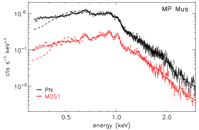
Fig. 3. PN (black) and MOS1 (red) spectra of MP Mus with superimposed the 3- T model (solid line) derived by Argiroffi et al. (2007) indicating low absorption ( N_{\text{H}} = 5 \times 10^{20} \text{ cm}^{-2} ), and the 3- T model (dashed line) obtained by fitting the EPIC spectra with an absorbing column fixed at 5 \times 10^{21} \text{ cm}^{-2} .
