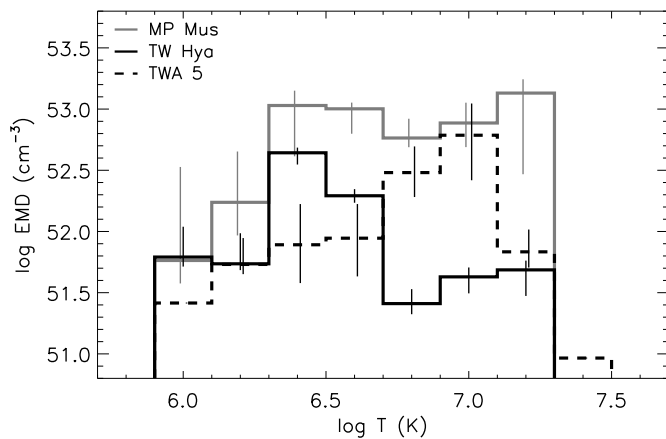
Fig. 6. Emission measure distributions derived from the RGS line fluxes.
