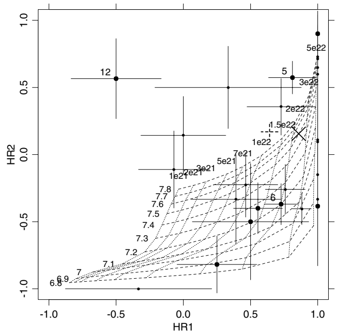
Fig. 5. Diagram of X-ray hardness ratios ( HR1, HR2 ), for all sources in the ACIS FOV, with error bars. Sources in the MWC 297 group are indicated by filled dots, among which we label with numbers the strongest two sources (X-ray #5 and #6), and MWC 297 (X-ray #12). The dashed error bars indicate the combined (ACIS) hardness ratios of the whole MWC 297 group. The dotted-dashed grid indicates predicted hardness ratios for single-temperature Raymond X-ray spectra, for various temperatures ( \log T = 6.8-7.8 \text{ K} ), and absorbing column densities ( N_H = 1 \times 10^{21}-5 \times 10^{22} \text{ cm}^{-2} ), as labeled. The thick X symbol corresponds to the predicted position according to the ASCA spectral parameters.
