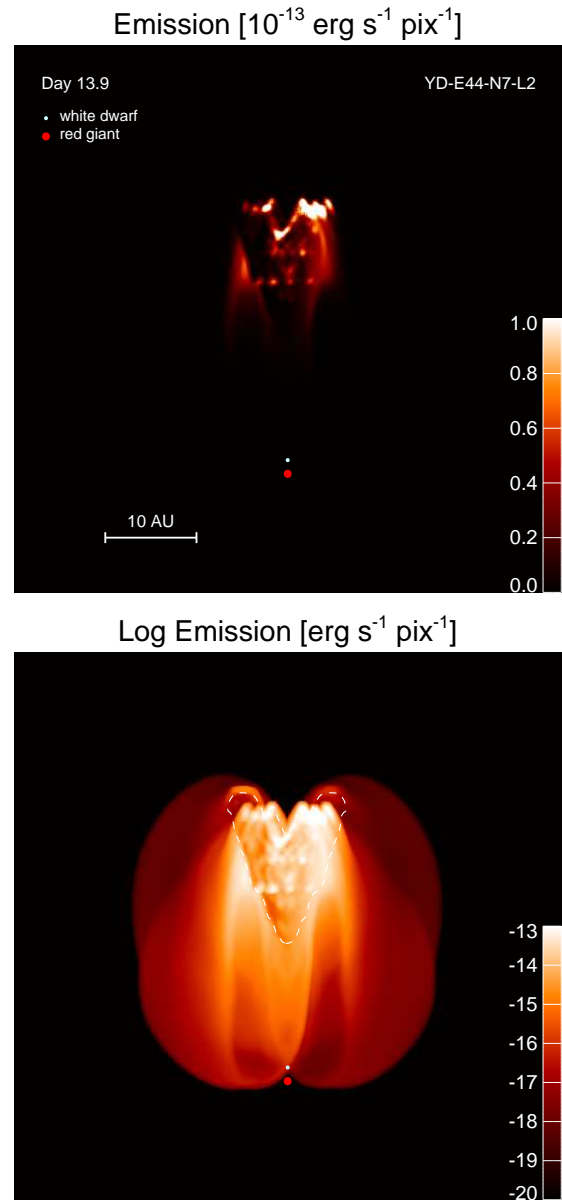
Figure 5. X-ray images in the [0.6 – 12.4] keV band in linear (upper panel) and logarithmic (lower panel) scales derived from model YD-E44-N7-L2 at day 13.9. The plane of the orbit of the central binary system lies on the (y, z) plane and is assumed to be inclined by 35^\circ to the line-of-sight (Dobrzycka & Kenyon 1994). The dashed contour encloses the ejecta material leading to the largest photoelectric absorption.
