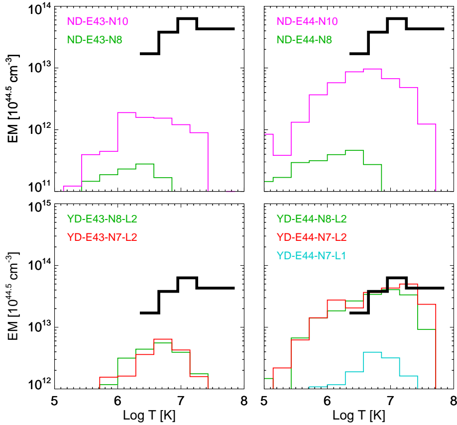
Figure 3. Emission measure vs. temperature distribution, EM(T) , of the blast wave at day 13.9. Upper panels show the result for models without EDE, lower panels for models with EDE. The black histogram represents the average EM(T) estimated from the analysis of Chandra /HETG observations (Drake et al. 2008). The factor 10^{44.5} assumes a distance for RS Oph of 1.6 kpc.
