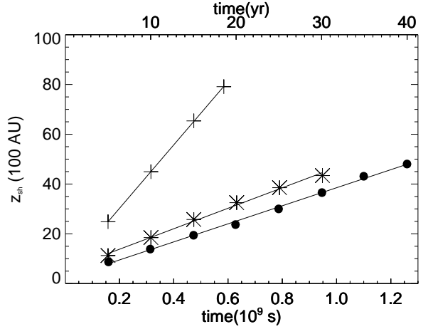
Figure 6. Shock front position vs. time. Dots mark the light jet case, stars the equal-density jet, and crosses the heavy jet case. The lines refer to the best fit, from which we derive the average shock speed: v_{\text{sh}} \approx 500 \text{ km s}^{-1} , \approx 600 \text{ km s}^{-1} , \approx 1900 \text{ km s}^{-1} for the light, equal-density and heavy jet case, respectively.
