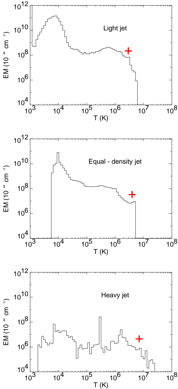
Figure 7. Emission measure, EM , as a function of the temperature, T for the three models discussed in the text, at a time 20 years after the beginning of the jet/ambient medium interaction. The cross superimposed on each panel marks the best-fit temperature and emission measure values derived from our simulated absorbed spectra.
