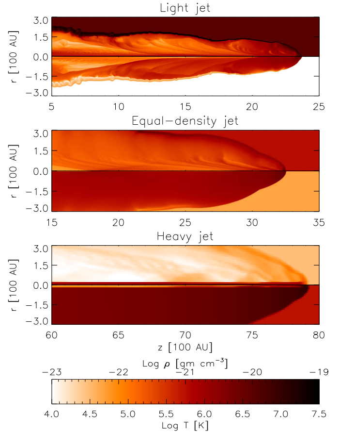
Figure 3. Two-dimensional mass density (upper half-panels) and temperature (lower half-panels) cuts in the r - z plane after 20 years since the beginning of the jet/ambient medium interaction for the best cases of light (upper panels), equal-density (middle panels) and heavy jets (lower panels).
