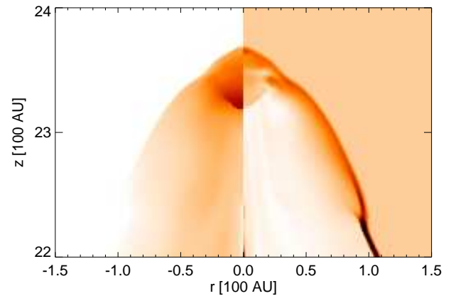
Figure 4. An enlargement of the post shock region in the light jet case for temperature (left) and density (right) in linear scale, obtained about 20 years after the beginning of the jet/ambient medium interaction. Note the hot and dense region just behind the shock front.
