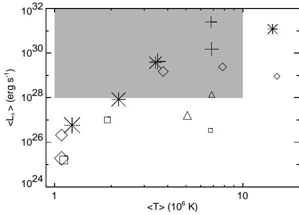
Figure 10. Mean value of the X-ray luminosity as a function of the mean value of the best fit temperature, derived from our model synthesized spectra. Crosses correspond to Mach number M = 1000 , stars to M = 300 , diamonds to M = 100 , triangles to M = 30 and squares to M = 10 . The increasing size of each symbol corresponds to increasing value of the ambient medium-to-jet density contrast, \nu = 0.01 -300. The shaded region refers to the (L_X, T) values consistent with observations of HH objects in general.
