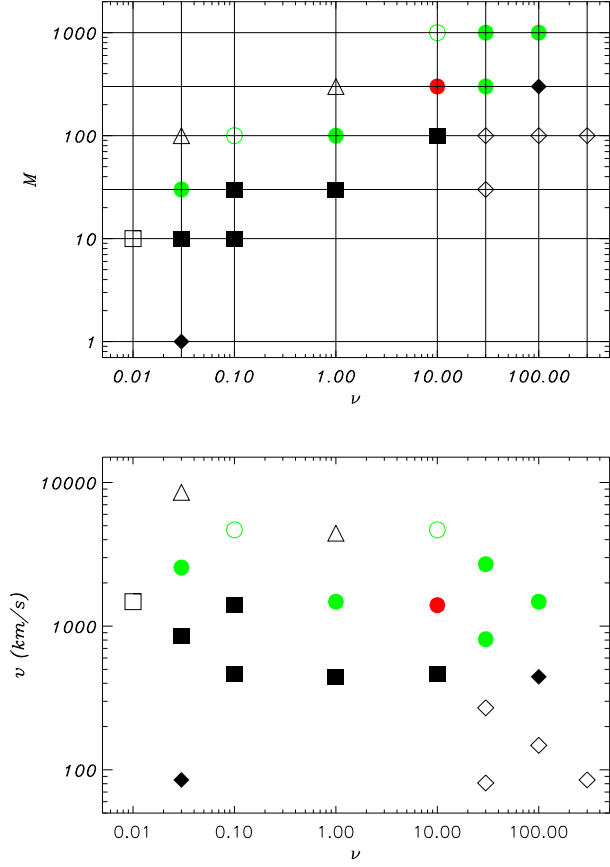
Figure 2. Exploration of the parameter space: jet Mach number, M (upper panel) and initial jet velocity (lower panel) as a function of the ambient-to-jet density contrast, \nu . Green and red dots refer to models consistent with observations for X-ray luminosity, shock velocity and fitting temperature values (see text); diamonds refer to models which cannot reproduce observations; squares refer to models in good agreement with observations for shock velocity but not for X-ray luminosity values; triangles refer to models with too high ( T \geq 10^7 K, one order of magnitude higher than observed) temperature. Empty symbols refer to pure hydrodynamic simulations; filled symbols refer to models in which thermal conduction and radiative losses effects are taken into account.
