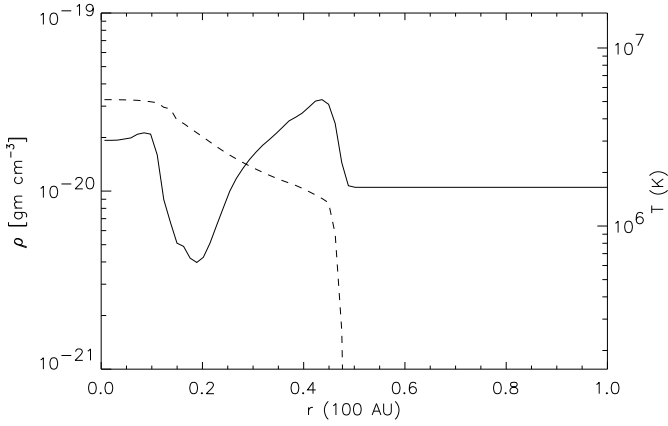
Figure 5. Density (continuous line) and temperature (dashed line) profiles along the radial direction at z \approx 5000 AU, corresponding to the blob position at t = 40 yr ( M = 300 , \nu = 10 ).
