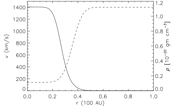
Figure 1. Initial jet velocity (continuous line) and density (dashed line) as a function of the distance from the axis, r , for the light jet case discussed in Section 3.2 with parameters: M = 300 , \nu = 10 , n_j = 500 \text{ cm}^{-3} , T_a = 10^3 \text{ K} , r_j = 30 \text{ AU} , w = 4 (see Table 3).
