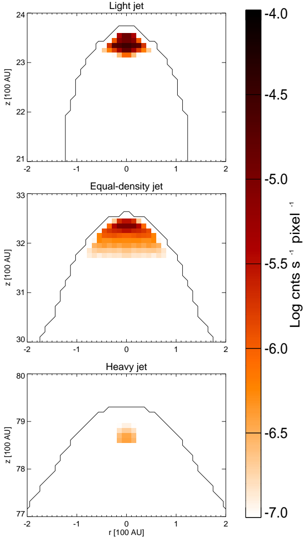
Figure 8. Synthesized X-ray emission, in logarithmic scale, as predicted to be observed with ACIS-I, for the three cases examined, 20 years since the beginning of the jet/ambient medium interaction. At a distance D \approx 150 pc, 100 AU corresponds to about 0.7 arcsec
