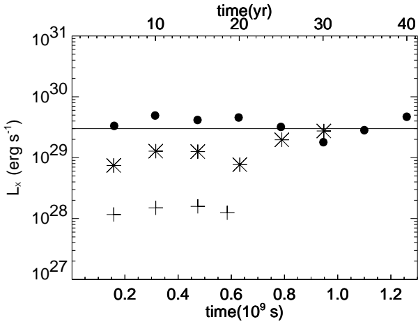
Figure 9. X-ray luminosity evolution as a function of time. Dots mark the light jet case, stars the equal-density jet, and crosses the heavy jet case. The line superimposed on this figure marks L_{\text{X}} 3 \times 10^{29} \text{ erg s}^{-1} , the value observed in HH 154 (Favata et al. 2002).
